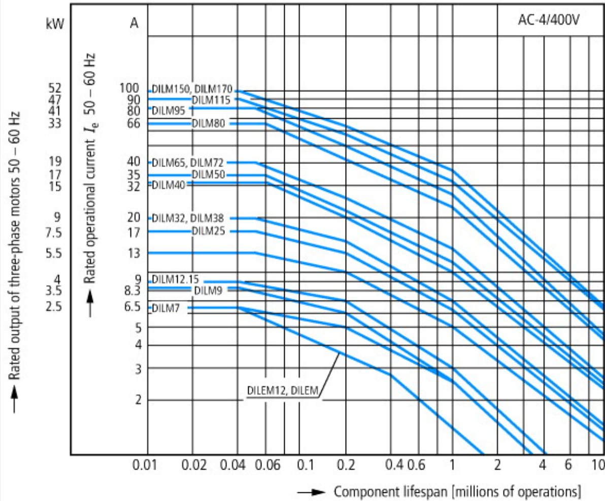
Characteristic curves
