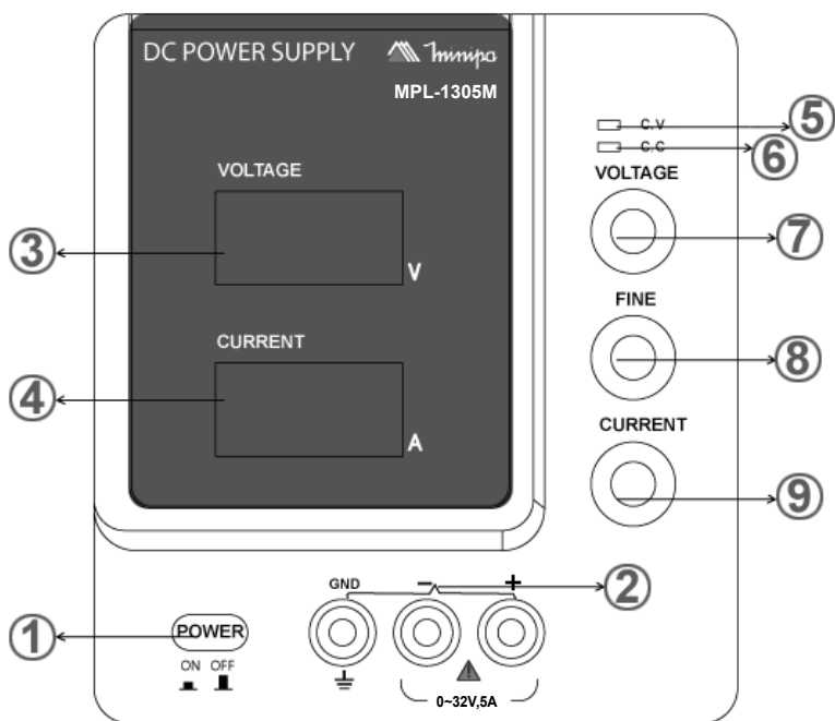
Figura 2 – Painel Frontal Fonte MPL-1305M
